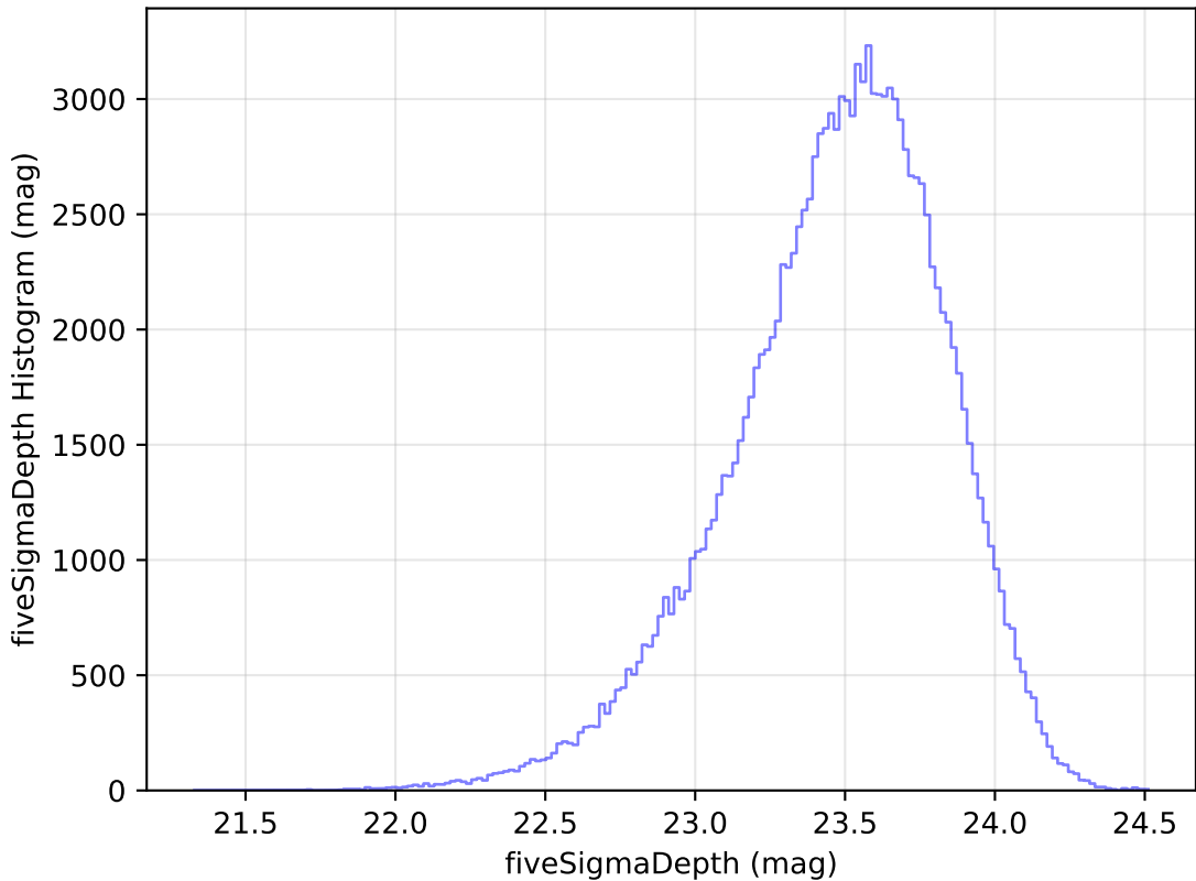
internal_u_expt45_nscale1.2v3.4_10yrs u: fiveSigmaDepth Histogram
