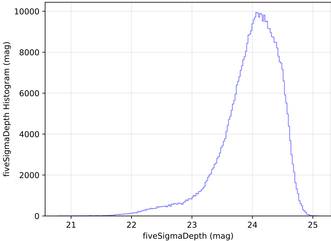
internal_u_expt45_nscale1.2v3.4_10yrs r: fiveSigmaDepth Histogram
