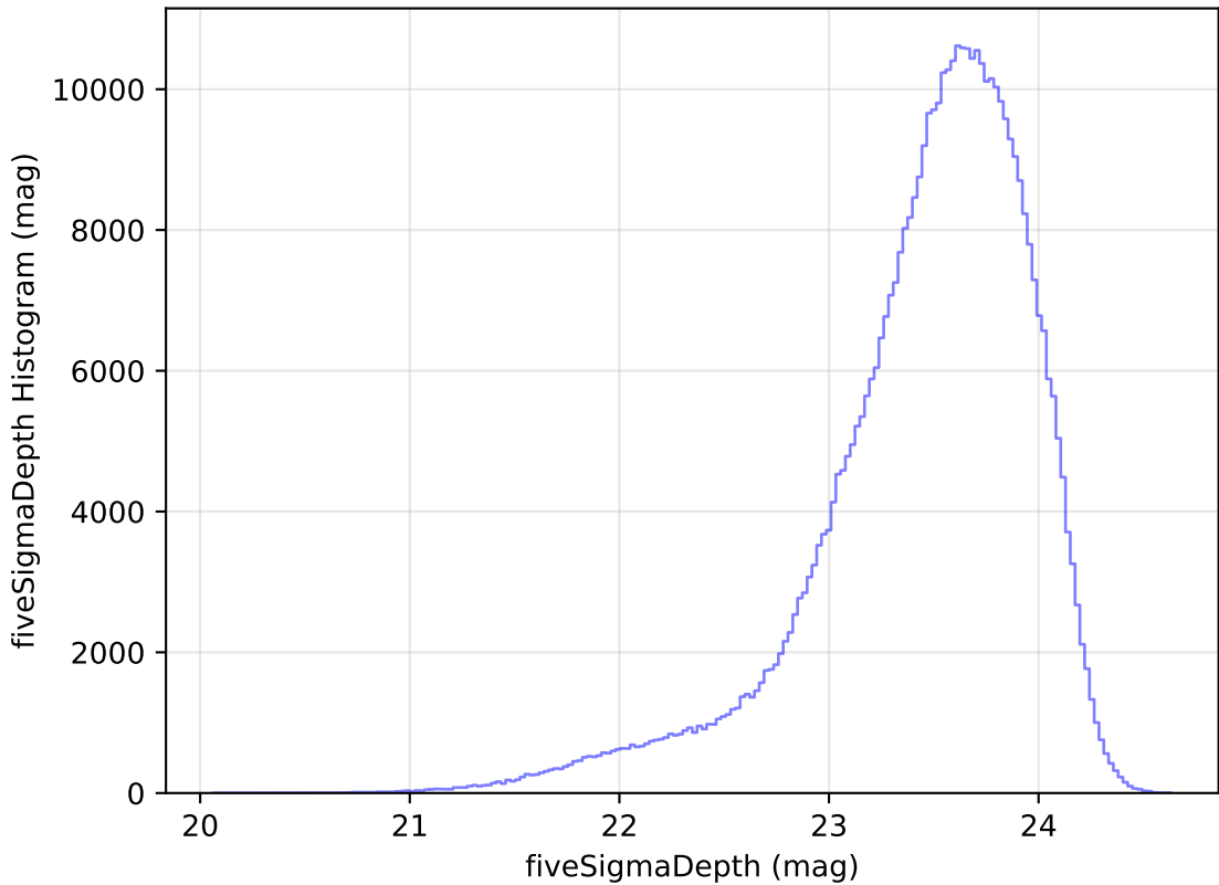
internal_u_expt45_nscale1.2v3.4_10yrs i: fiveSigmaDepth Histogram
