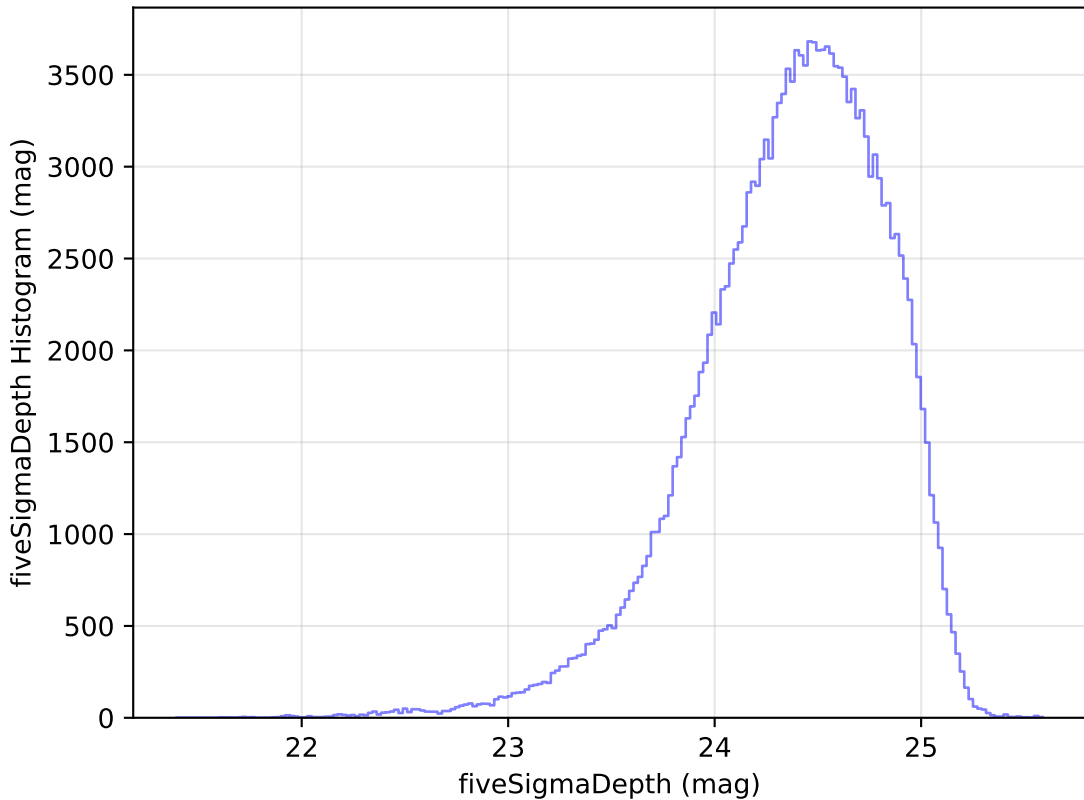
internal_u_expt45_nscale1.2v3.4_10yrs g: fiveSigmaDepth Histogram
