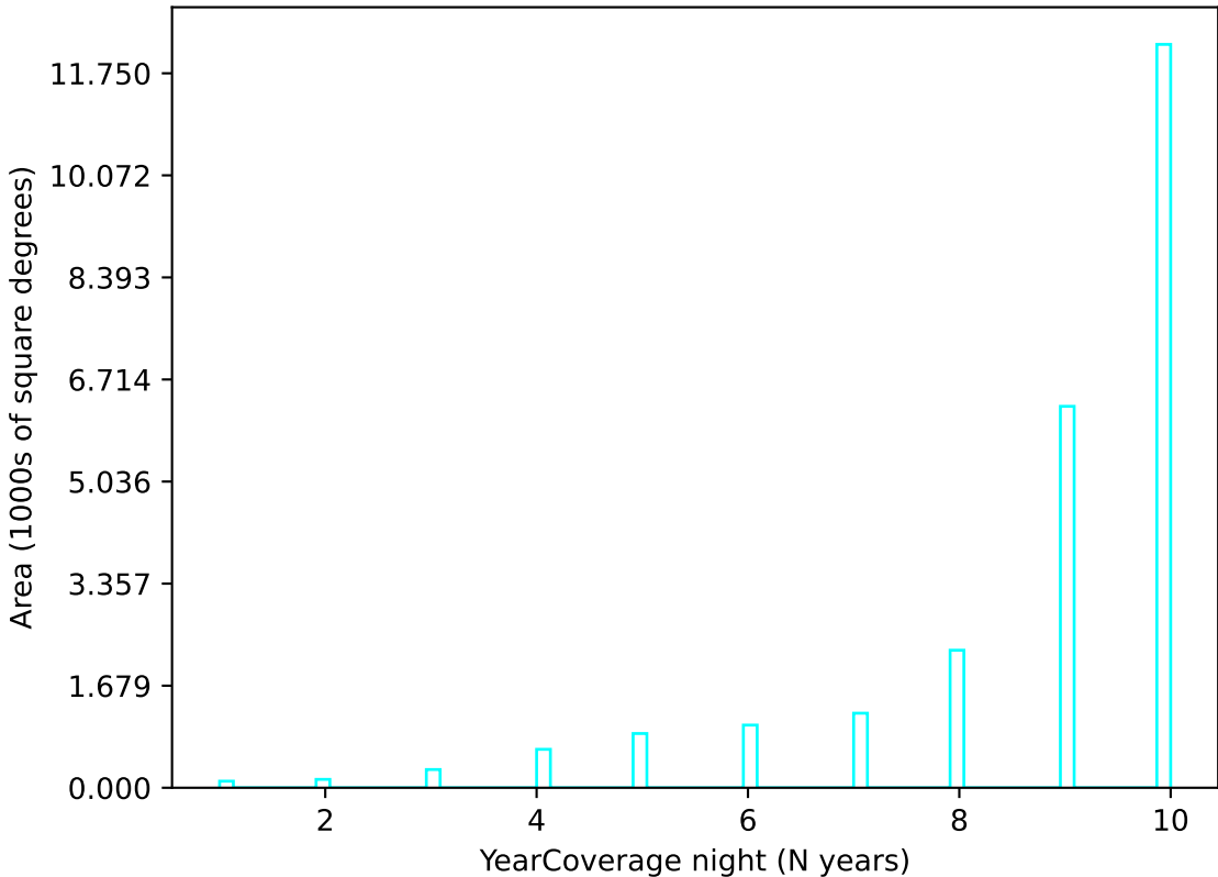
internal_u_expt45_nscale1.2v3.4_10yrs u band: YearCoverage night
