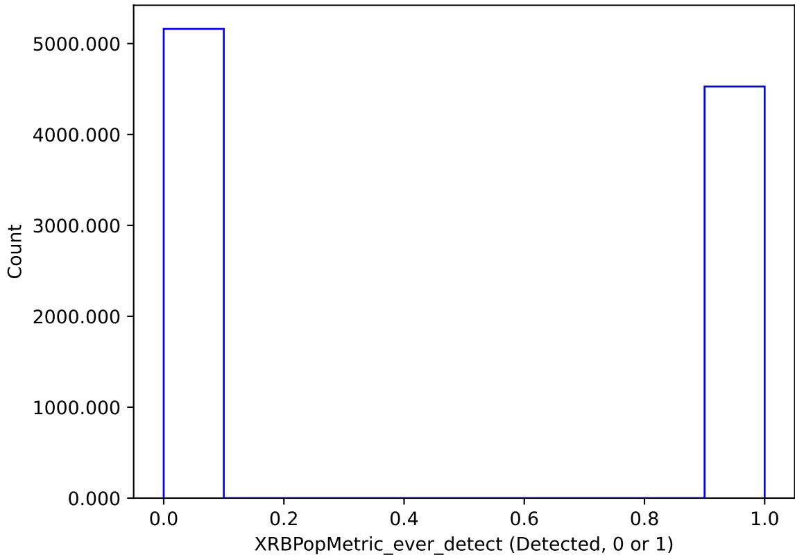
internal_u_expt45_nscale1.2v3.4_10yrs : XRBPoMetric_ever_detect
