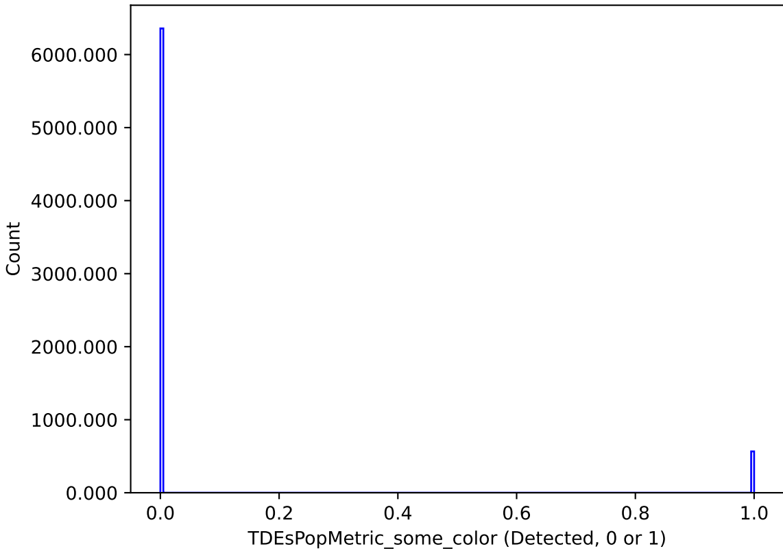
internal_u_expt45_nscale1.2v3.4_10yrs : TDEsPopMetric_some_color
