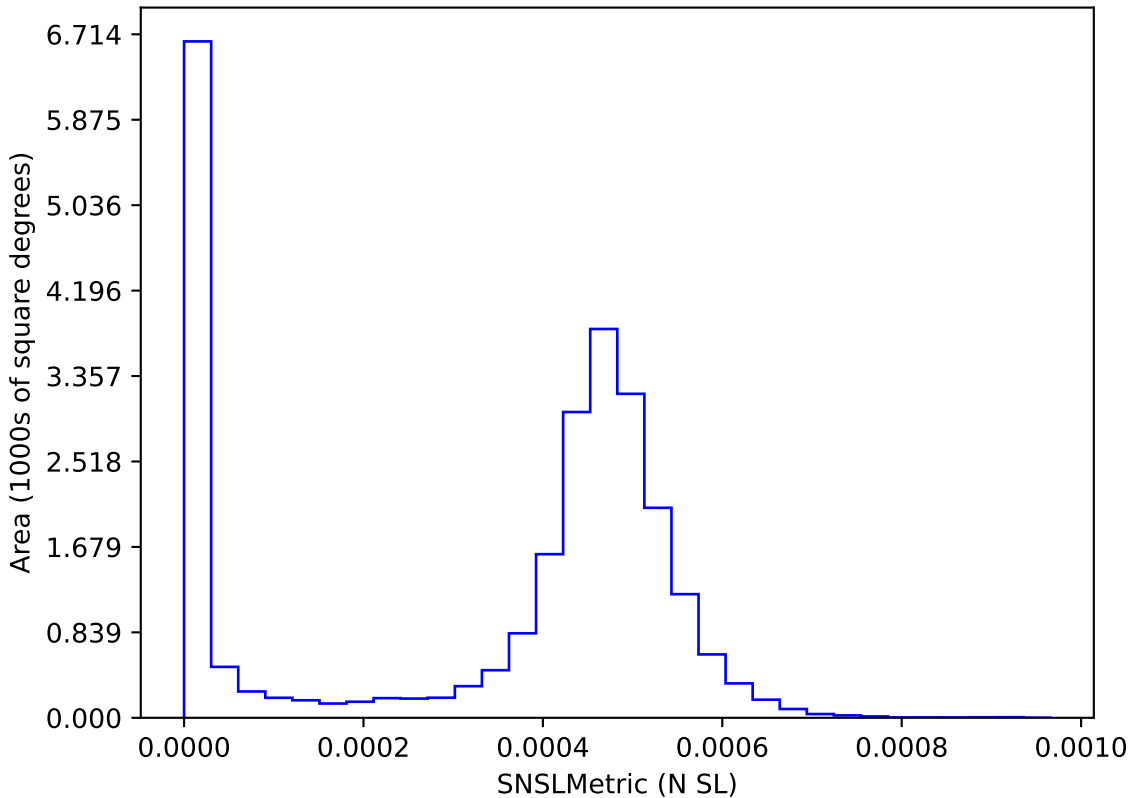
internal_u_expt45_nscale1.2v3.4_10yrs : SNSLMetric
