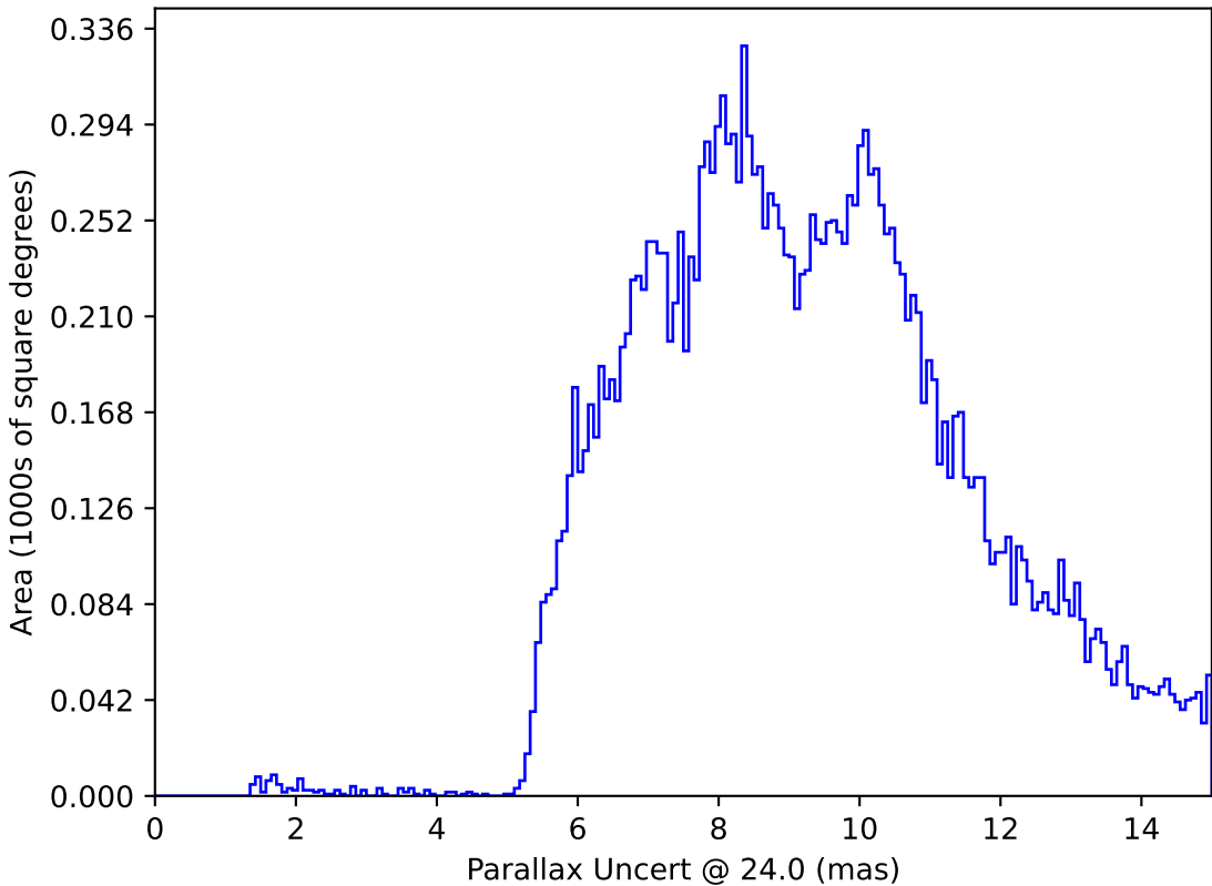
internal_u_expt45_nscale1.2v3.4_10yrs : Parallax Uncert @ 24.0
