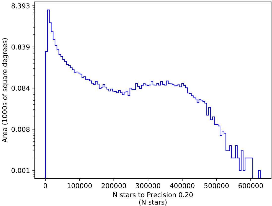
internal_u_expt45_nscale1.2v3.4_10yrs y: N stars to Precision 0.20
