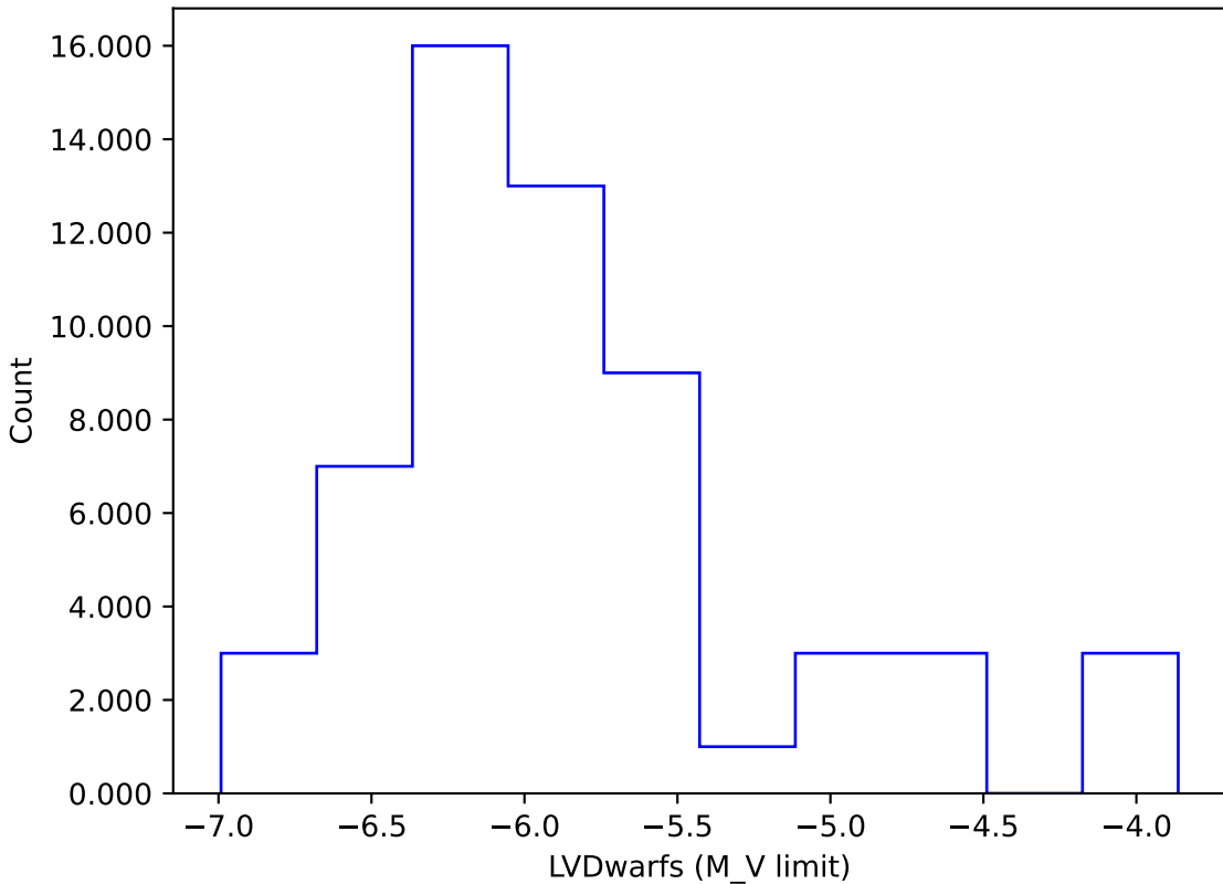
internal_u_expt45_nscale1.2v3.4_10yrs gi: LVDwarfs
