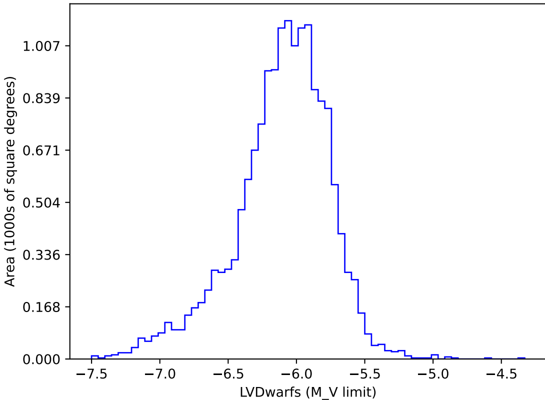
internal_u_expt45_nscale1.2v3.4_10yrs gi: LVDwarfs
