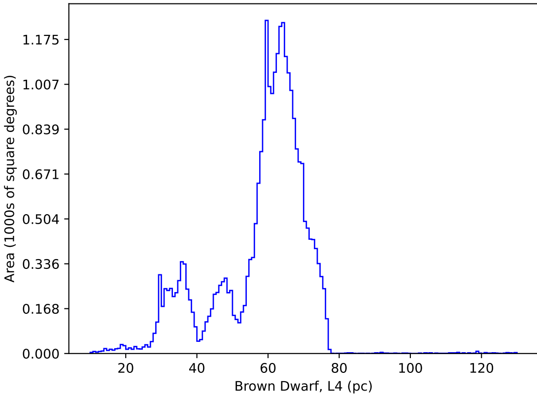
internal_u_expt45_nscale1.2v3.4_10yrs : Brown Dwarf, L4
