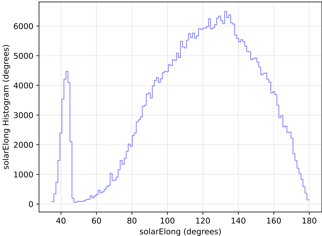
internal_u_expt45_nscale1.2v3.4_10yrs WFD z band: solarElong Histogram
