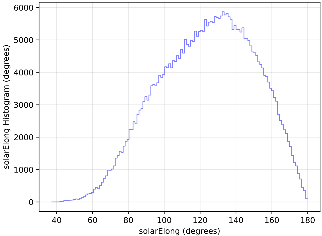
internal_u_expt45_nscale1.2v3.4_10yrs WFD y band: solarElong Histogram
