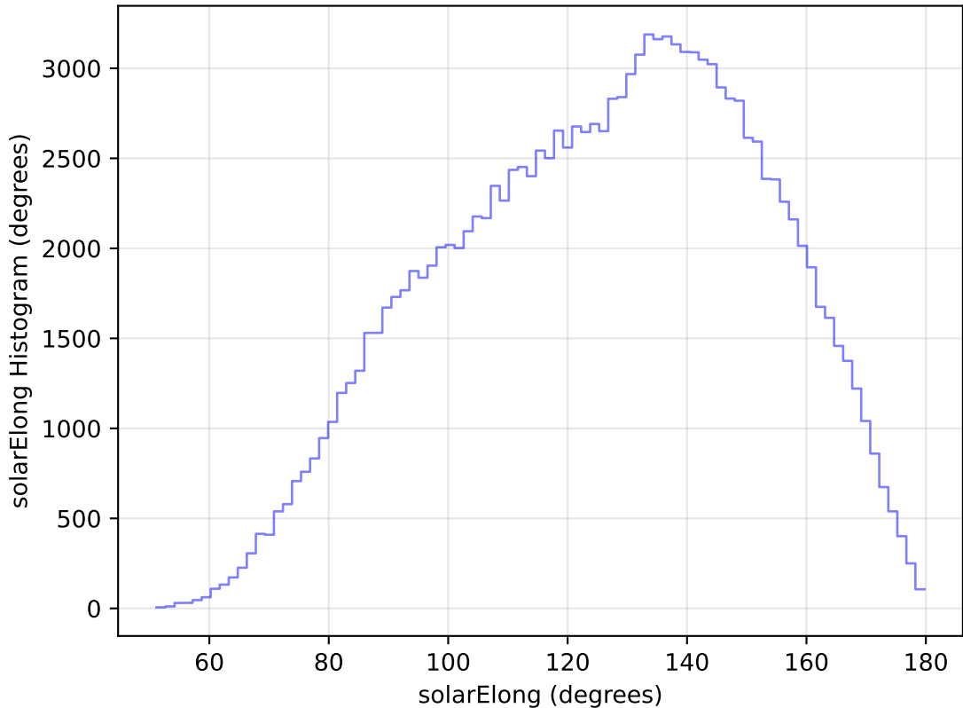
internal_u_expt45_nscale1.2v3.4_10yrs WFD u band: solarElong Histogram
