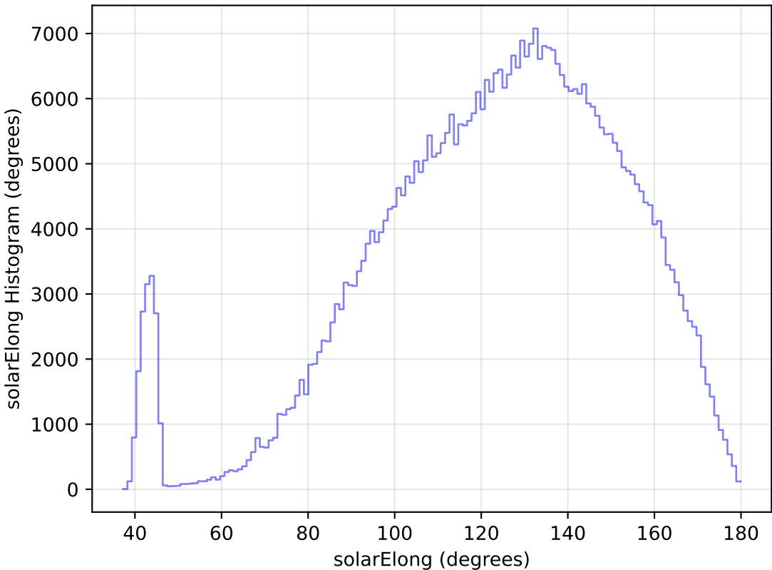
internal_u_expt45_nscale1.2v3.4_10yrs WFD r band: solarElong Histogram
