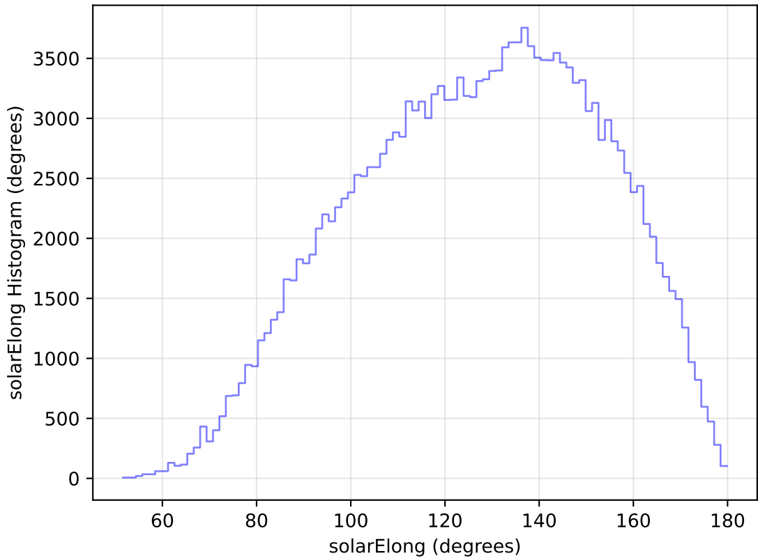
internal_u_expt45_nscale1.2v3.4_10yrs WFD g band: solarElong Histogram
