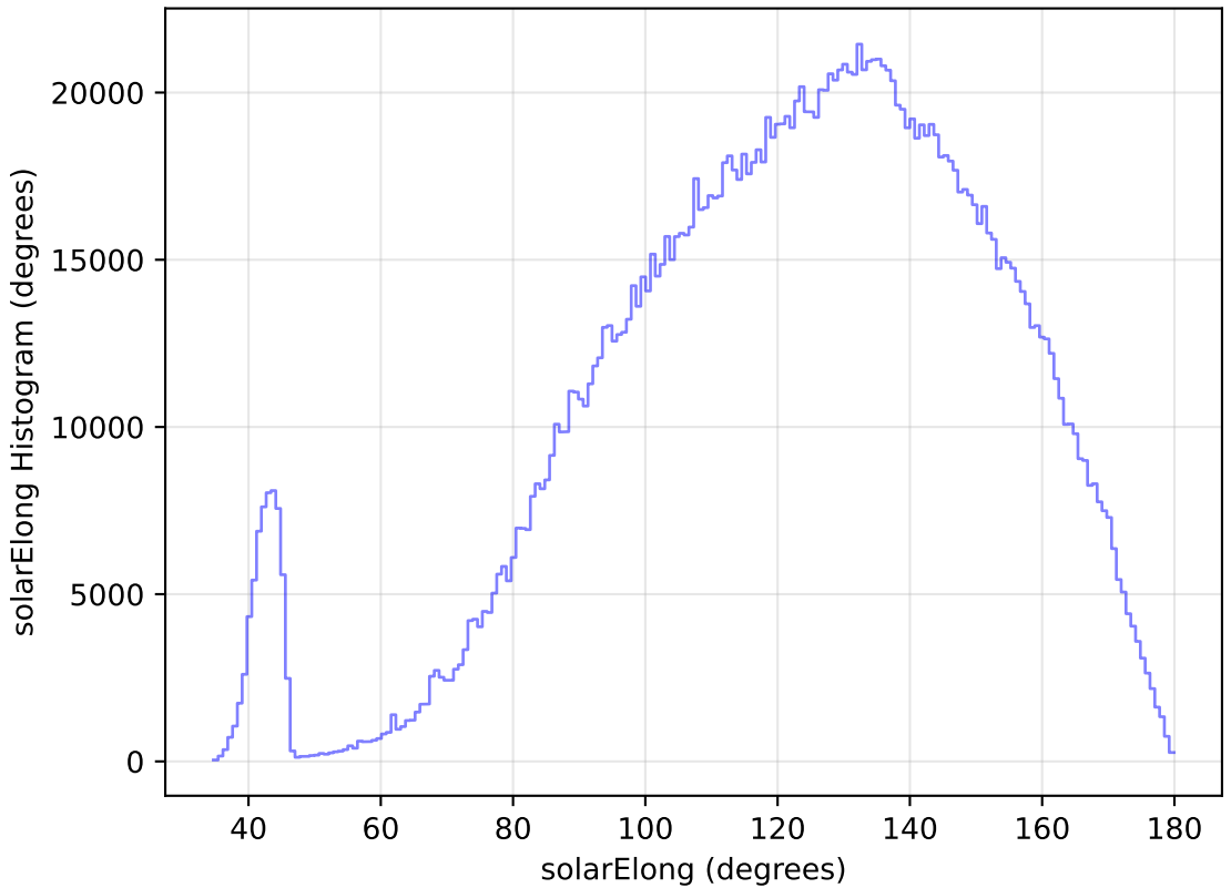
internal_u_expt45_nscale1.2v3.4_10yrs WFD all bands: solarElong Histogram
