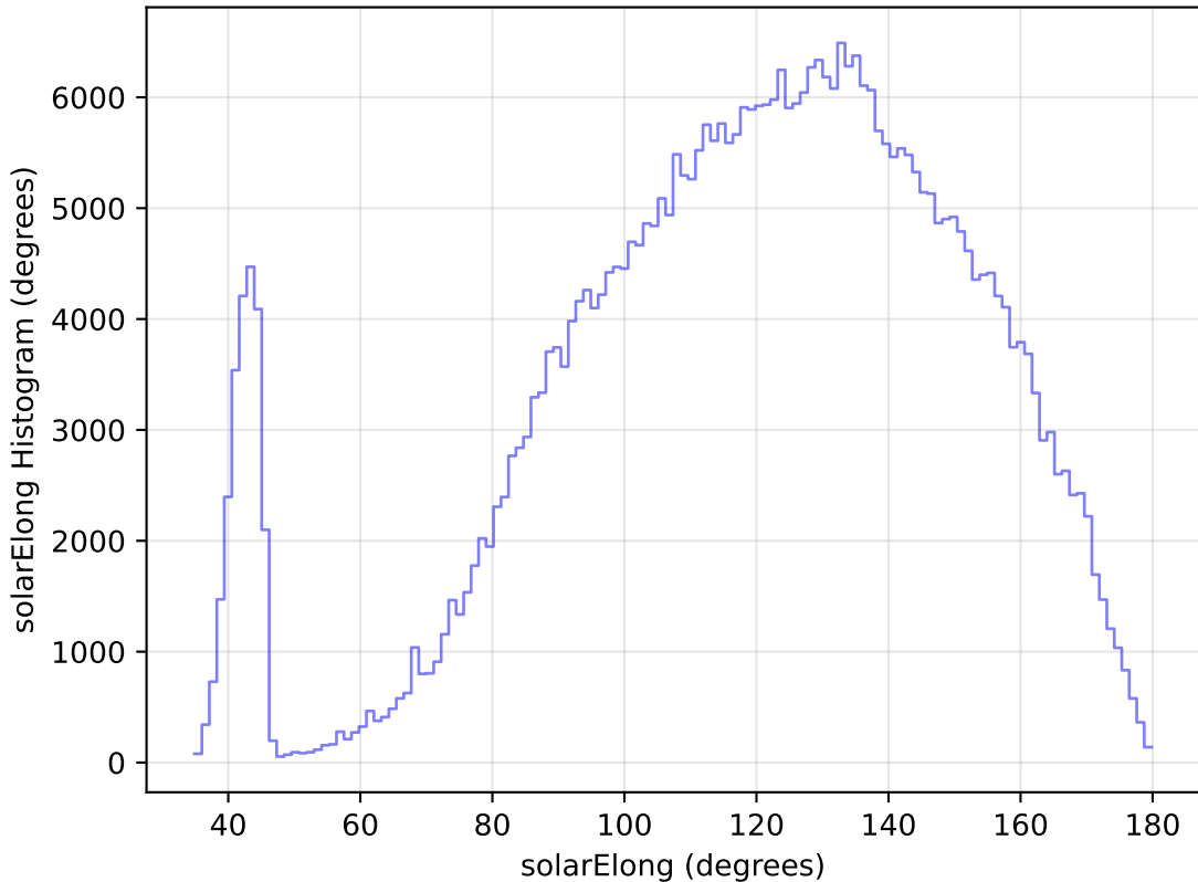
internal_u_expt45_nscale1.2v3.4_10yrs All sky z band: solarElong Histogram
