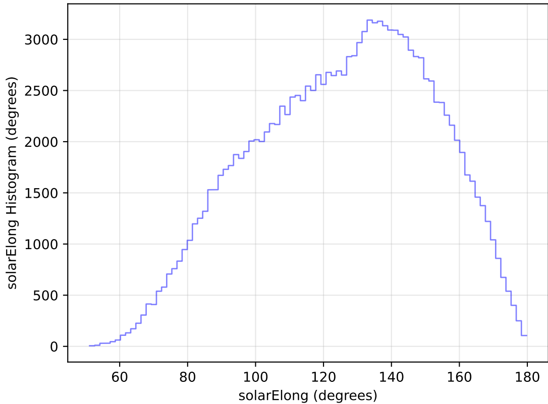
internal_u_expt45_nscale1.2v3.4_10yrs All sky u band: solarElong Histogram
