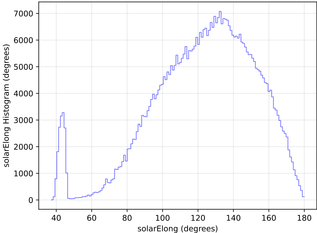
internal_u_expt45_nscale1.2v3.4_10yrs All sky r band: solarElong Histogram
