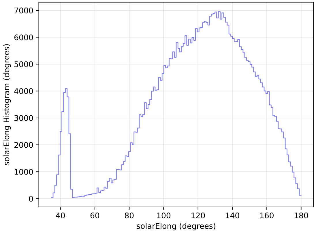
internal_u_expt45_nscale1.2v3.4_10yrs All sky i band: solarElong Histogram
