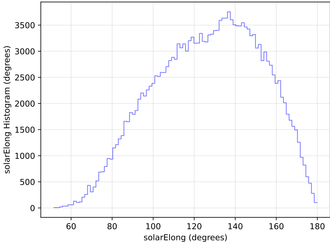
internal_u_expt45_nscale1.2v3.4_10yrs All sky g band: solarElong Histogram
