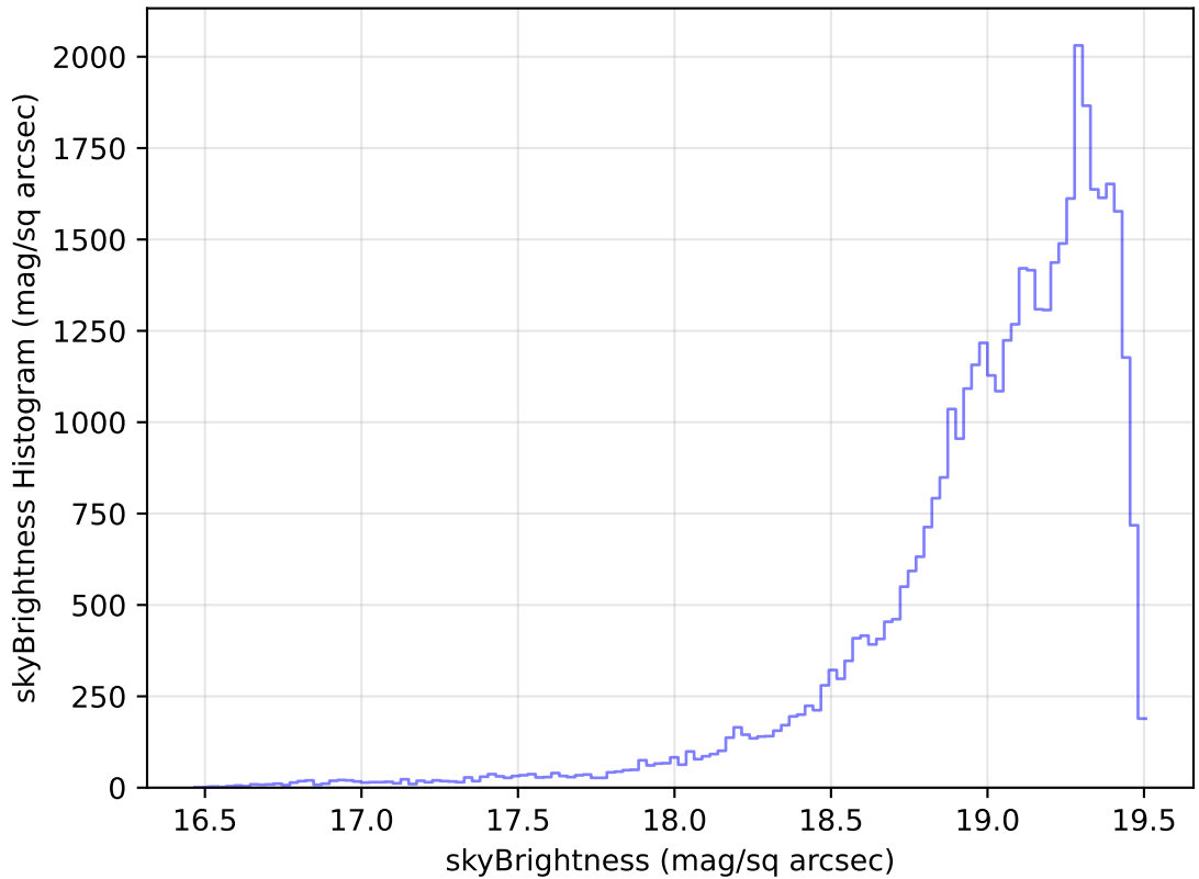
internal_u_expt45_nscale1.2v3.4_10yrs Yr 1 z band: skyBrightness Histogram
