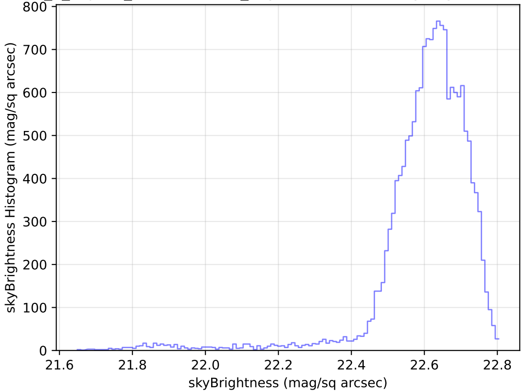
internal_u_expt45_nscale1.2v3.4_10yrs Yr 1 u band: skyBrightness Histogram
