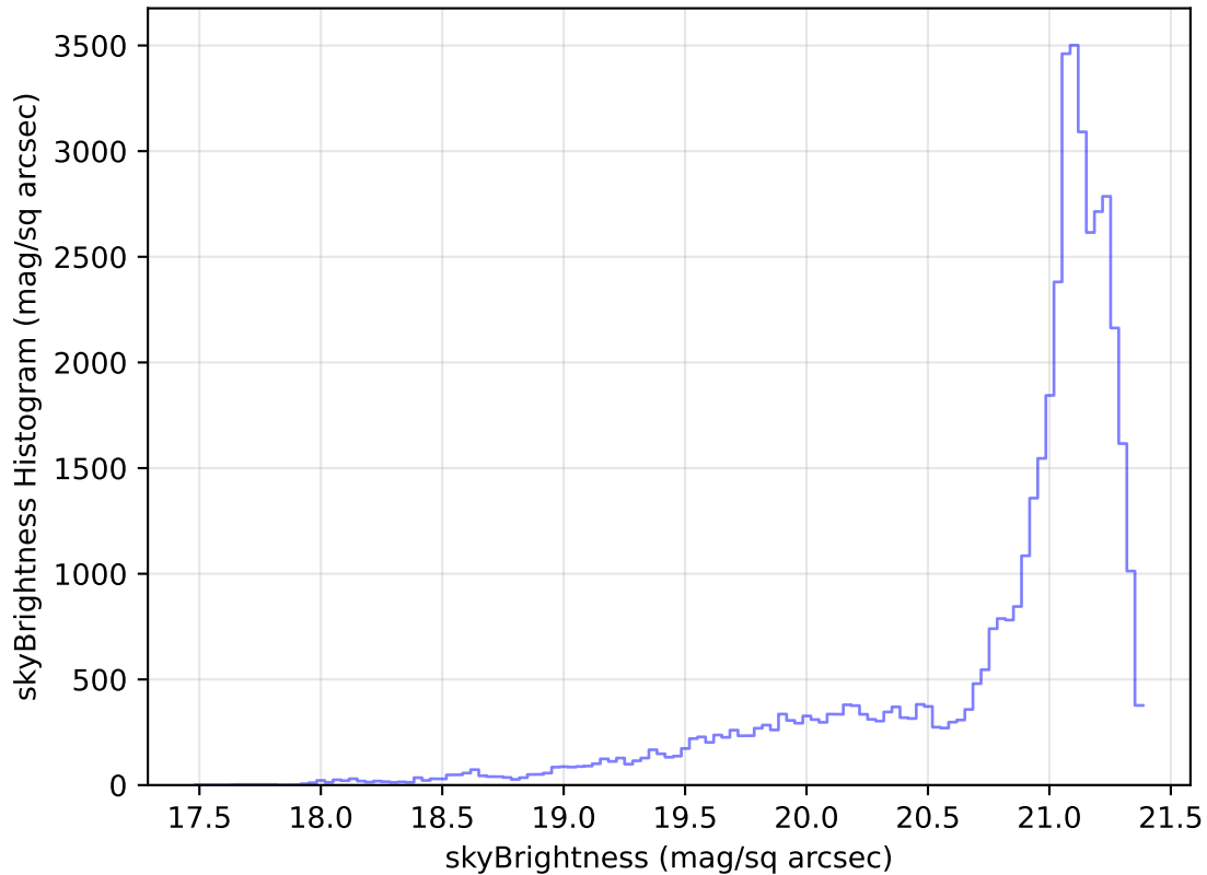
internal_u_expt45_nscale1.2v3.4_10yrs Yr 1 r band: skyBrightness Histogram
