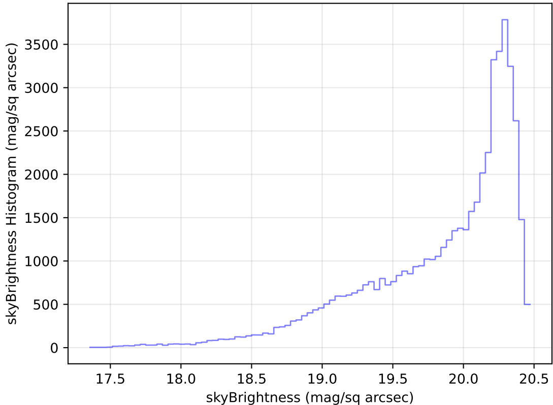
internal_u_expt45_nscale1.2v3.4_10yrs Yr 1 i band: skyBrightness Histogram
