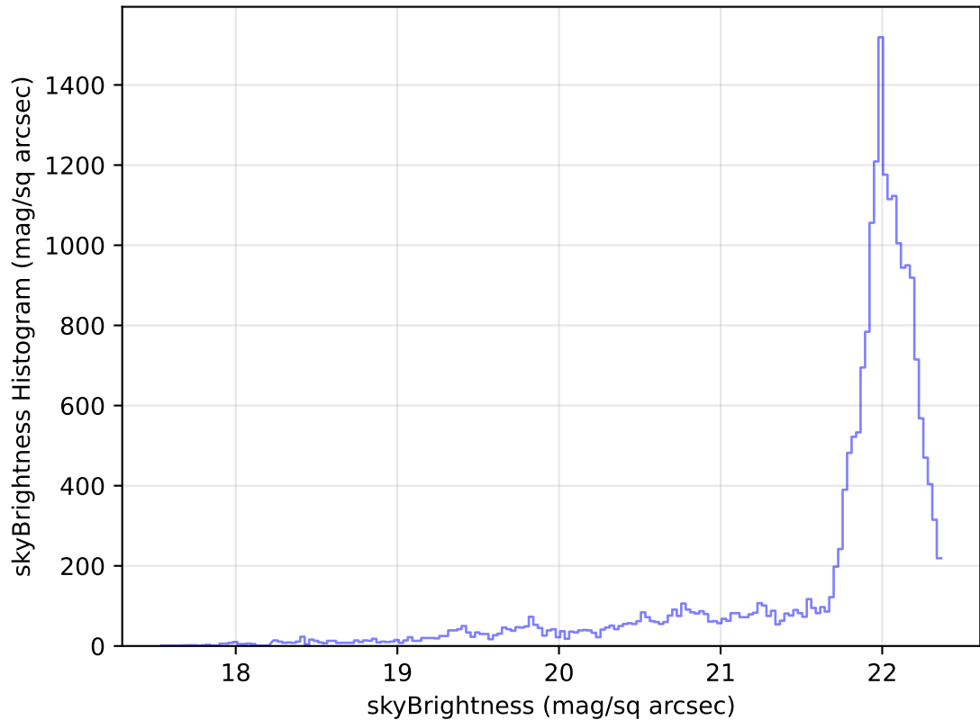
internal_u_expt45_nscale1.2v3.4_10yrs Yr 1 g band: skyBrightness Histogram
