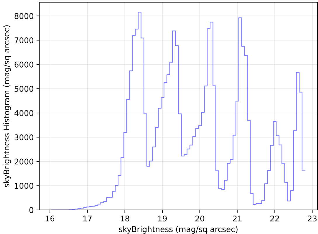
internal_u_expt45_nscale1.2v3.4_10yrs Yr 1 all bands: skyBrightness Histogram
