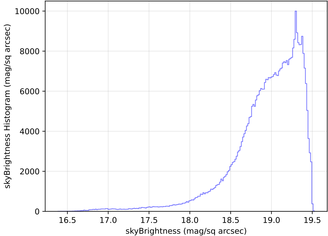
internal_u_expt45_nscale1.2v3.4_10yrs WFD z band: skyBrightness Histogram
