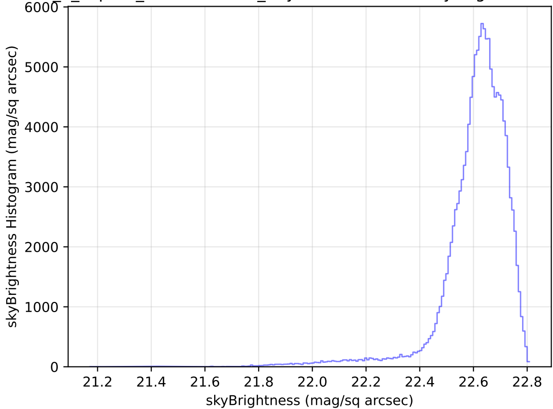
internal_u_expt45_nscale1.2v3.4_10yrs WFD u band: skyBrightness Histogram
