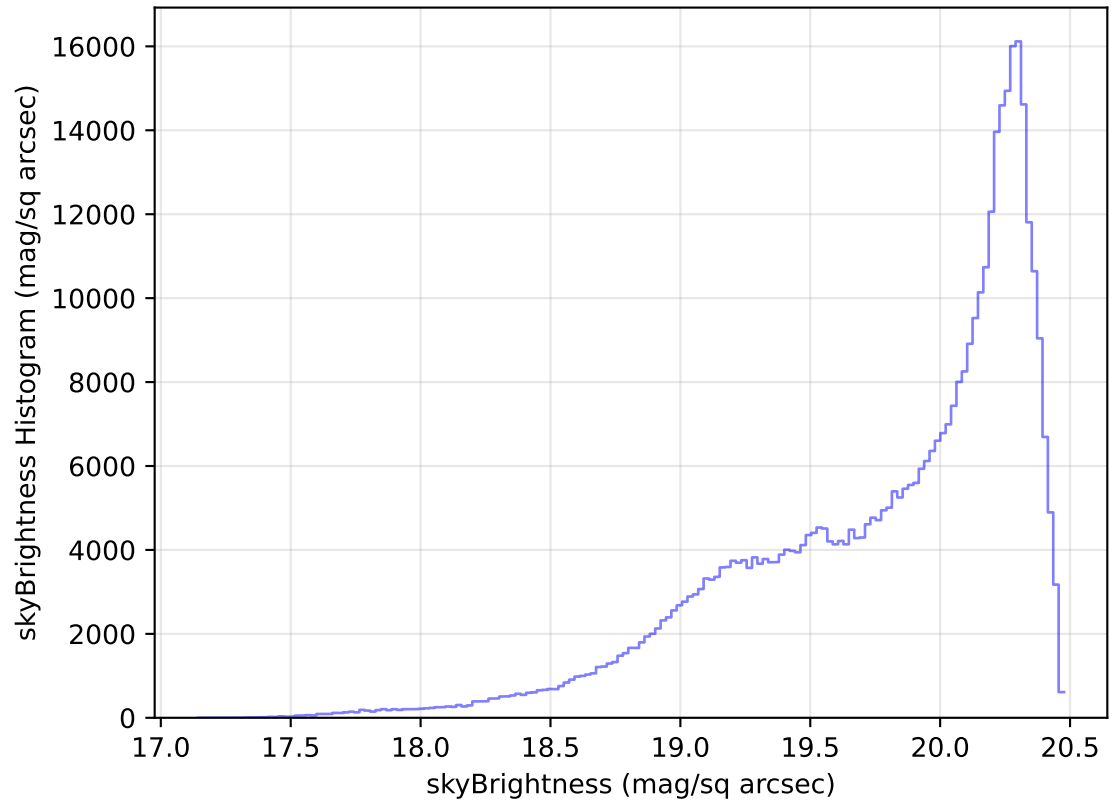
internal_u_expt45_nscale1.2v3.4_10yrs WFD i band: skyBrightness Histogram
