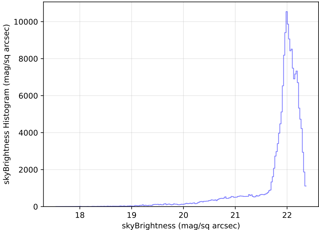
internal_u_expt45_nscale1.2v3.4_10yrs WFD g band: skyBrightness Histogram
