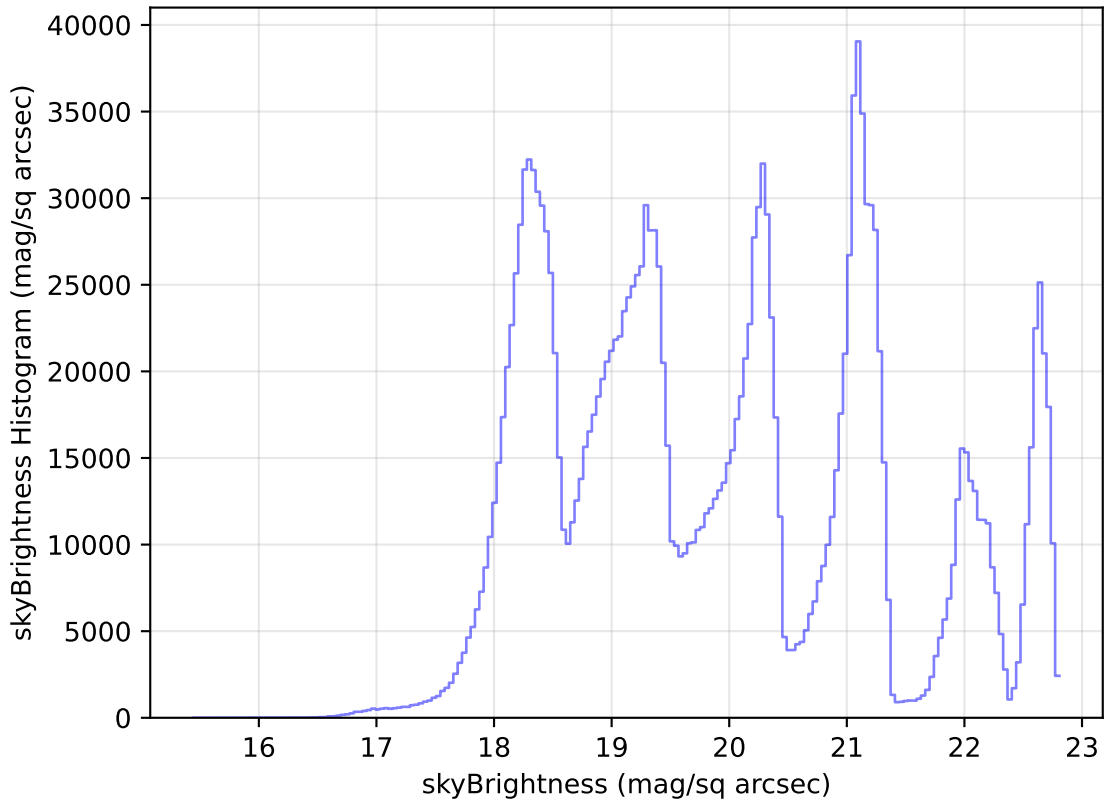
internal_u_expt45_nscale1.2v3.4_10yrs WFD all bands: skyBrightness Histogram
