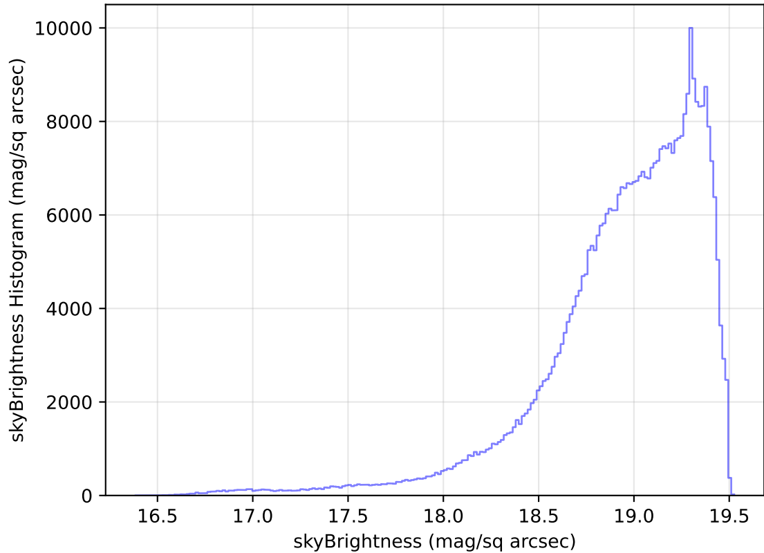
internal_u_expt45_nscale1.2v3.4_10yrs All sky z band: skyBrightness Histogram
