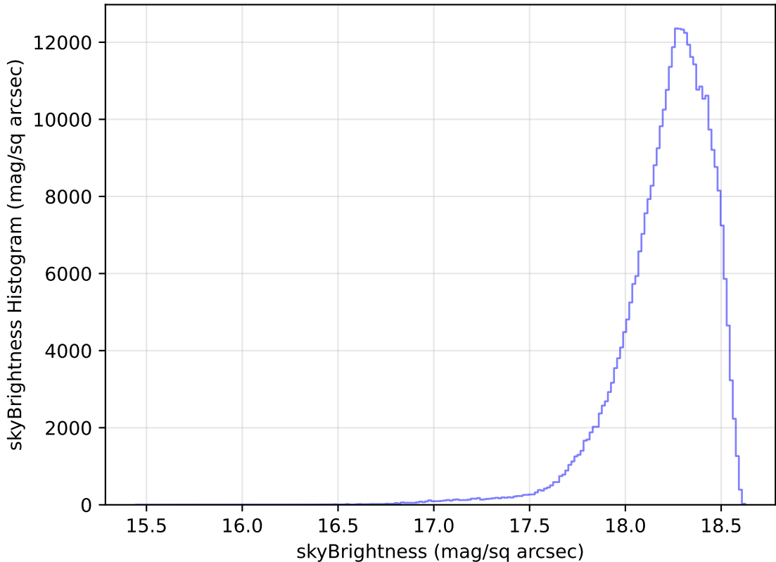
internal_u_expt45_nscale1.2v3.4_10yrs All sky y band: skyBrightness Histogram
