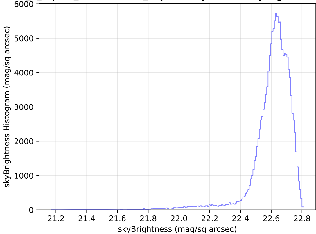
internal_u_expt45_nscale1.2v3.4_10yrs All sky u band: skyBrightness Histogram
