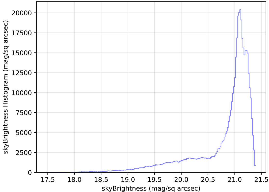
internal_u_expt45_nscale1.2v3.4_10yrs All sky r band: skyBrightness Histogram
