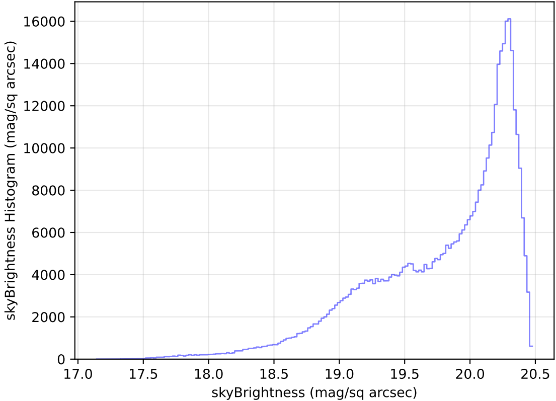
internal_u_expt45_nscale1.2v3.4_10yrs All sky i band: skyBrightness Histogram
