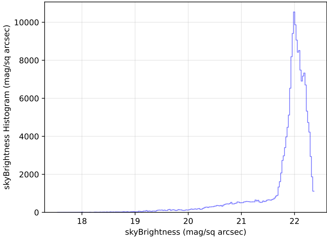
internal_u_expt45_nscale1.2v3.4_10yrs All sky g band: skyBrightness Histogram
