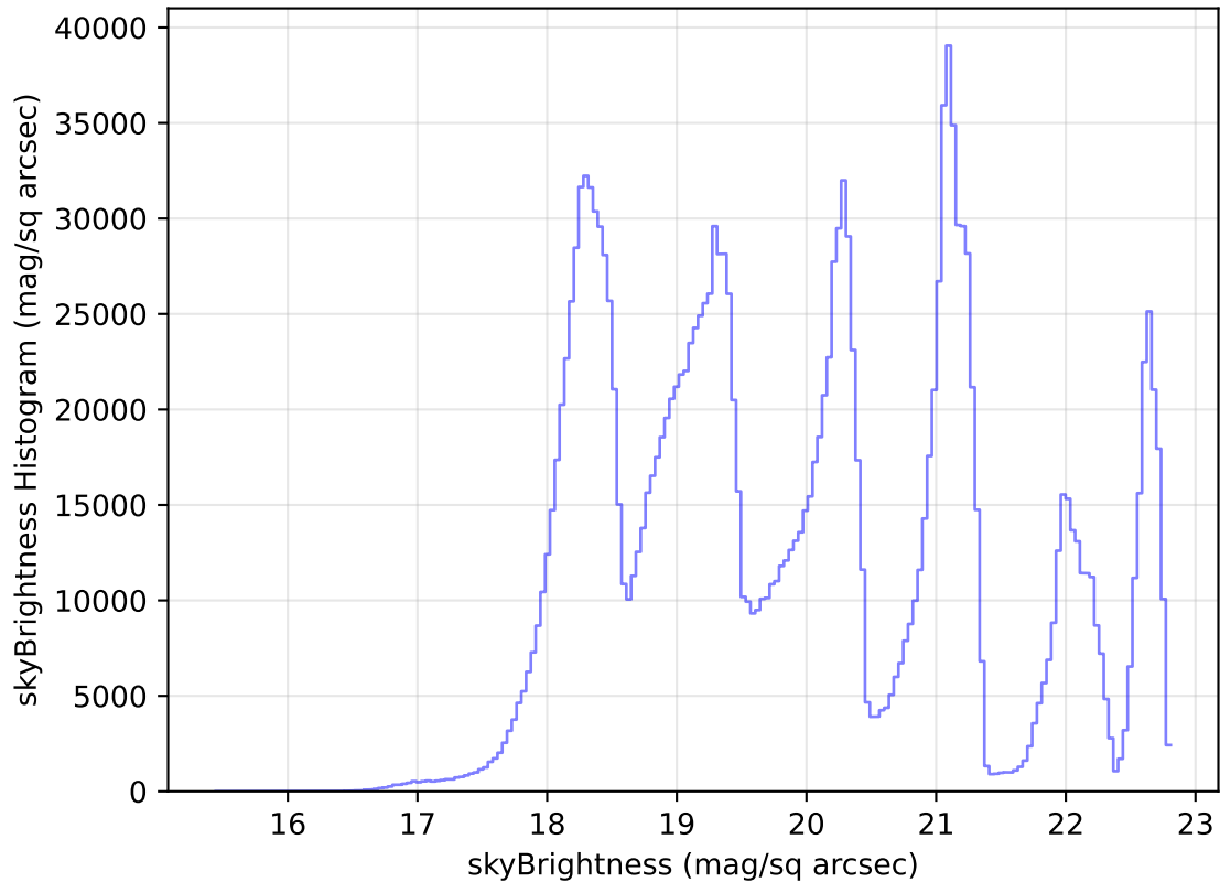
internal_u_expt45_nscale1.2v3.4_10yrs All sky all bands: skyBrightness Histogram
