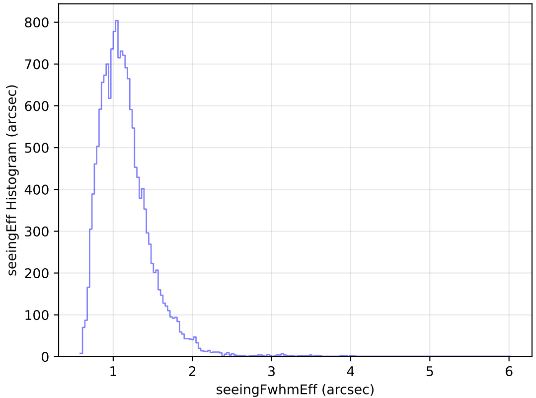
internal_u_expt45_nscale1.2v3.4_10yrs Yr 1 u band: seeingEff Histogram
