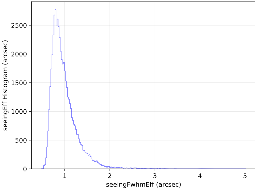
internal_u_expt45_nscale1.2v3.4_10yrs Yr 1 i band: seeingEff Histogram
