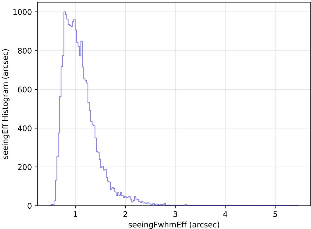
internal_u_expt45_nscale1.2v3.4_10yrs Yr 1 g band: seeingEff Histogram
