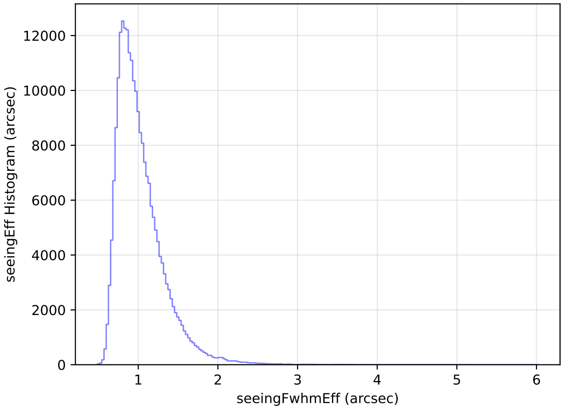
internal_u_expt45_nscale1.2v3.4_10yrs Yr 1 all bands: seeingEff Histogram
