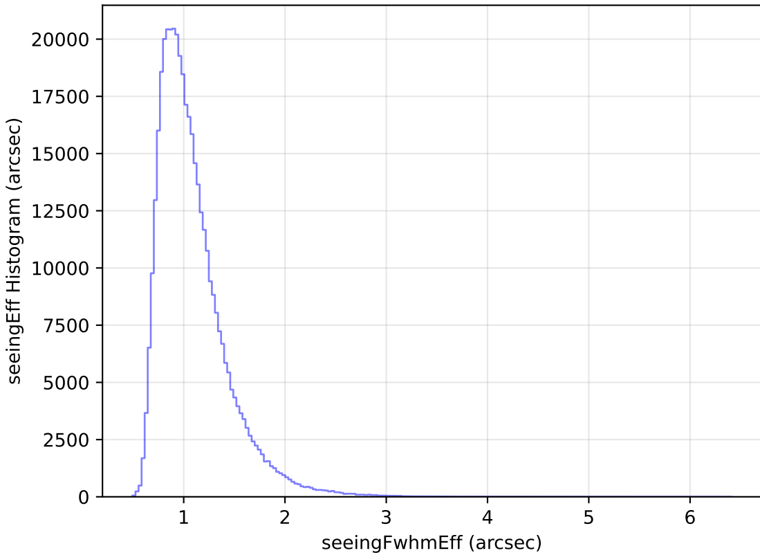
internal_u_expt45_nscale1.2v3.4_10yrs WFD z band: seeingEff Histogram
