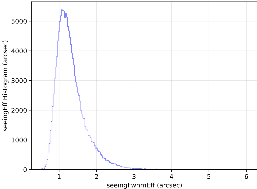
internal_u_expt45_nscale1.2v3.4_10yrs WFD u band: seeingEff Histogram
