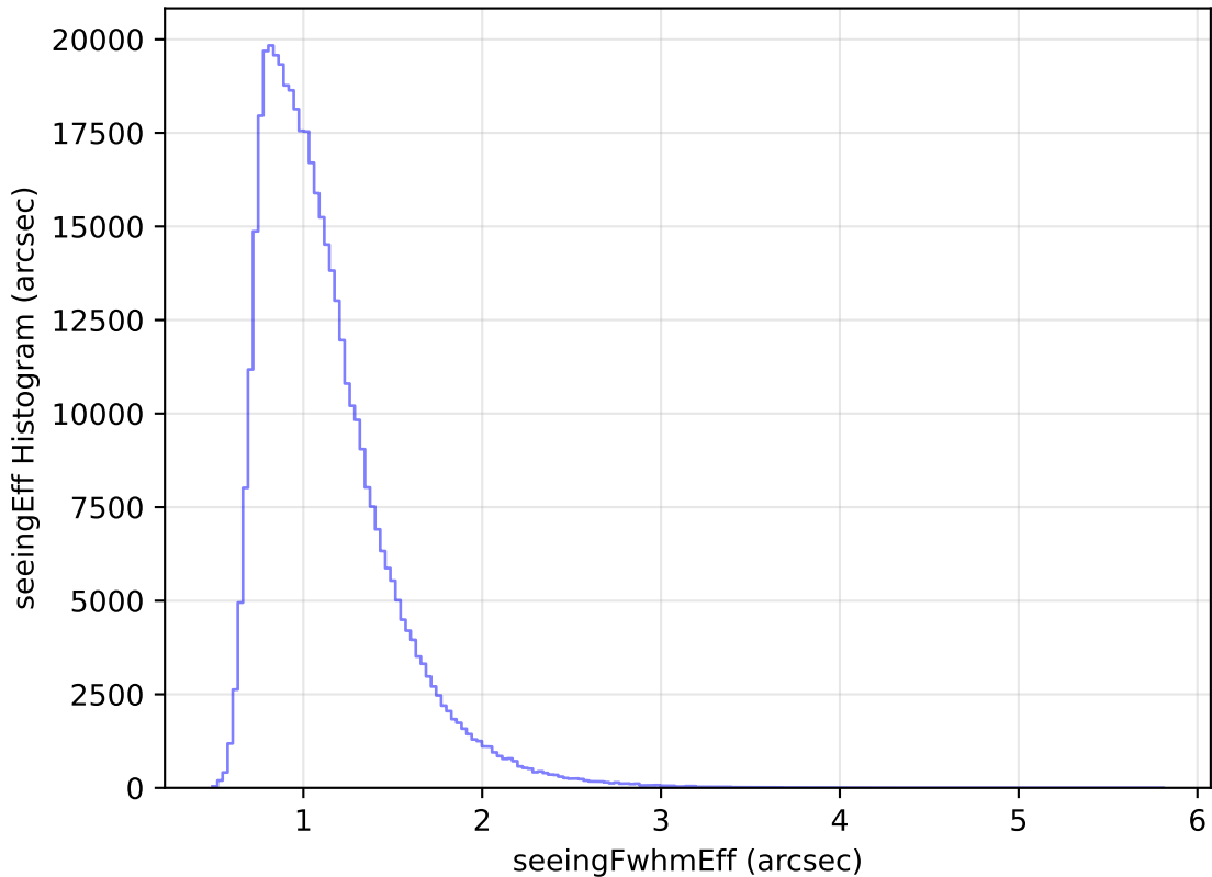
internal_u_expt45_nscale1.2v3.4_10yrs WFD r band: seeingEff Histogram
