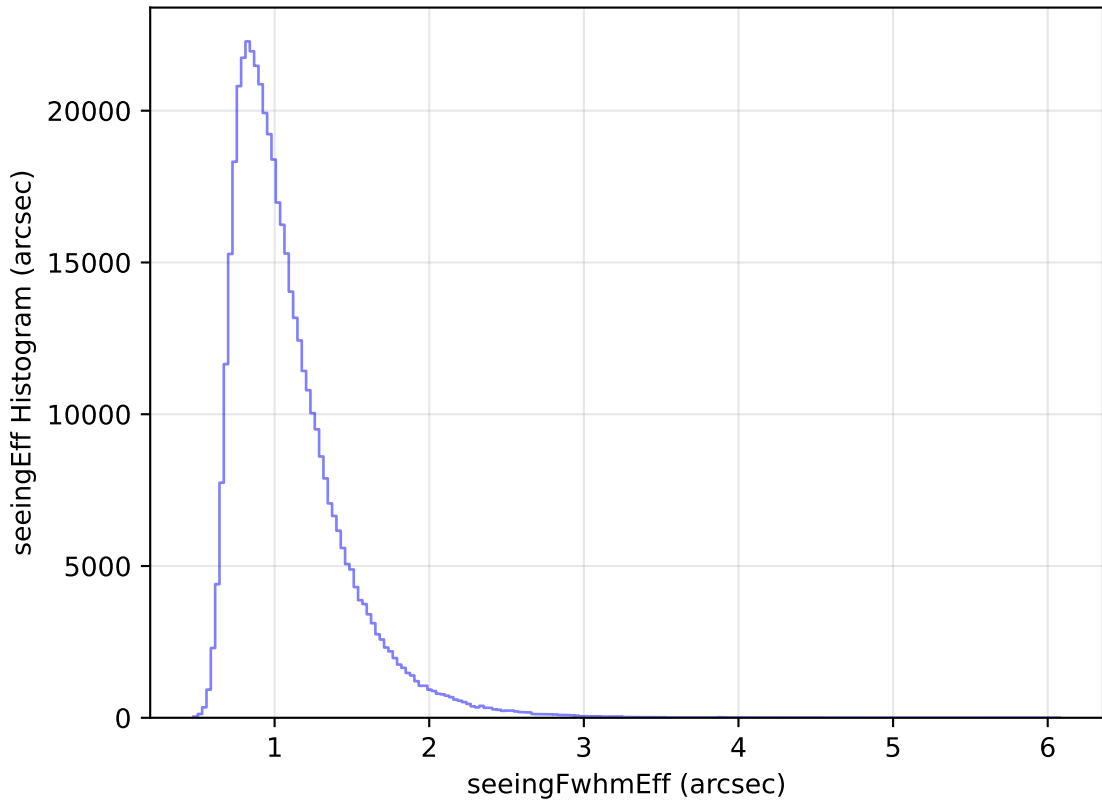
internal_u_expt45_nscale1.2v3.4_10yrs WFD i band: seeingEff Histogram
